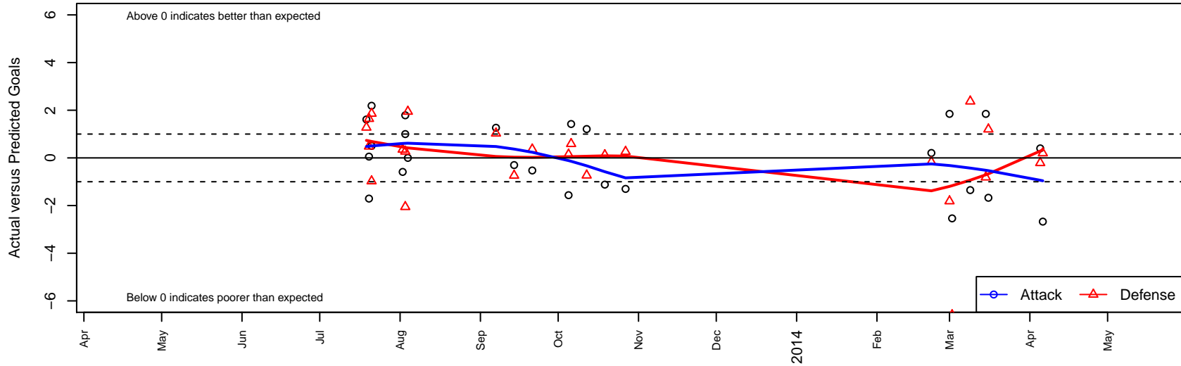
Albany FC Arsenal B99 Dots are actual minus expected GF (blue circles) and GA (red triangles). Blue line is smoothed change in attack strength. Red is smoothed change in defense strength.
